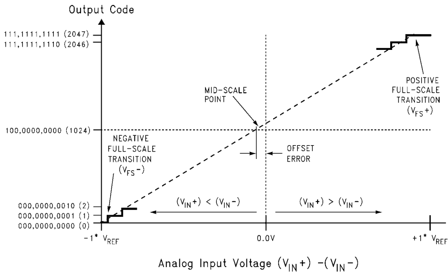
FIGURE 1. Transfer Characteristic (Offset Binary Format)
